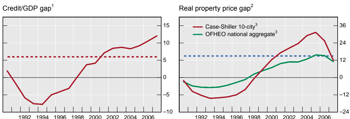
Graph A.1 Estimated gaps for the United States
