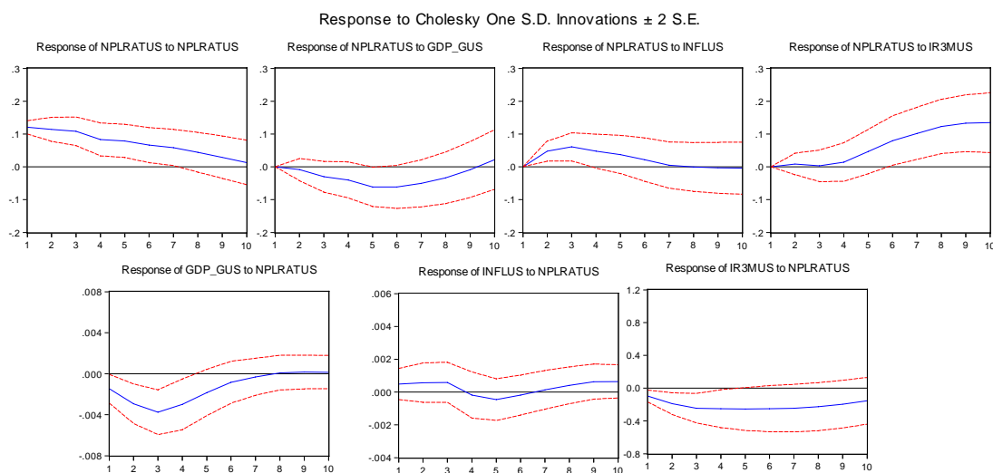
Graph II. 5 Impulse response functions of a FS VAR for the US 1
